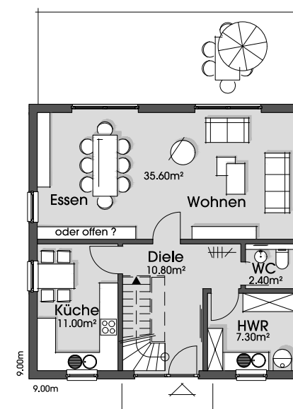
Erdgeschoss 1:175 67.10 m 2
